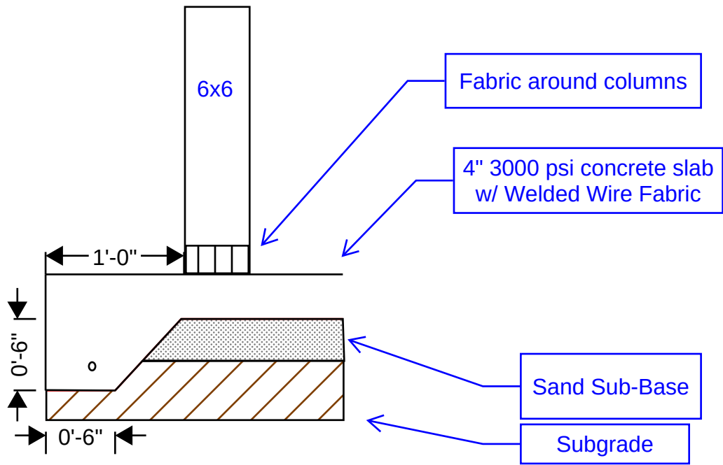
Section View
